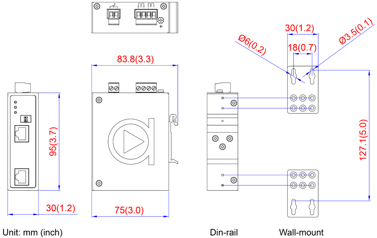
Figure 2.1 - Physical Dimensions
