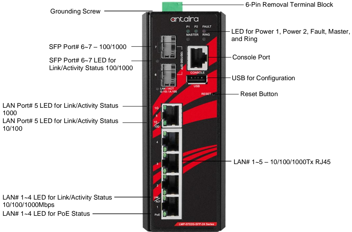
Figure 2.2 - The Front Panel of LMP-0702G-SFP-24-V2 Series
