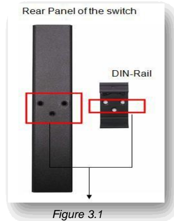
Figure 3.1 The Rear Side of the Switch and DIN-
